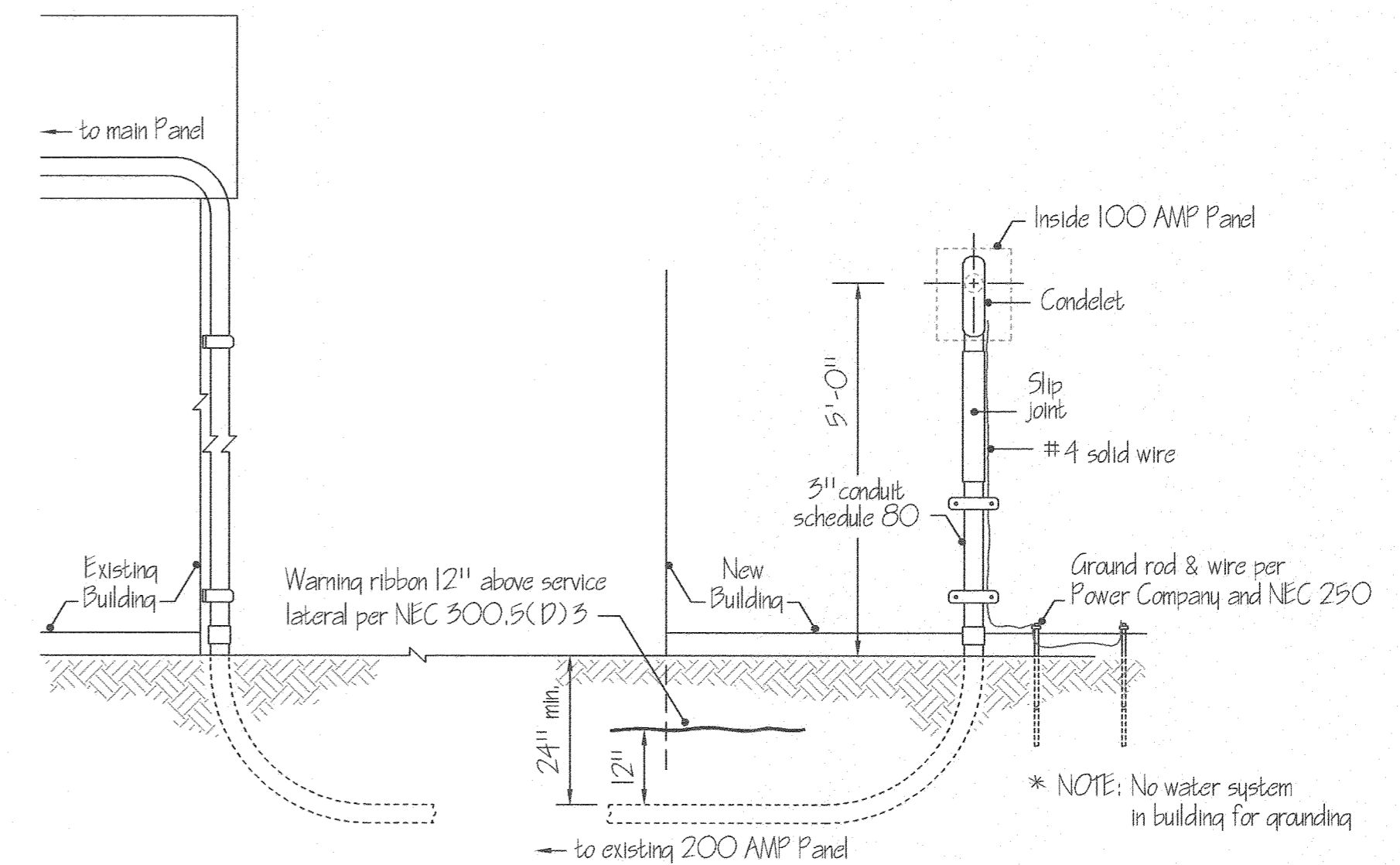
SERVICE DETAIL NOT TO SCALE
