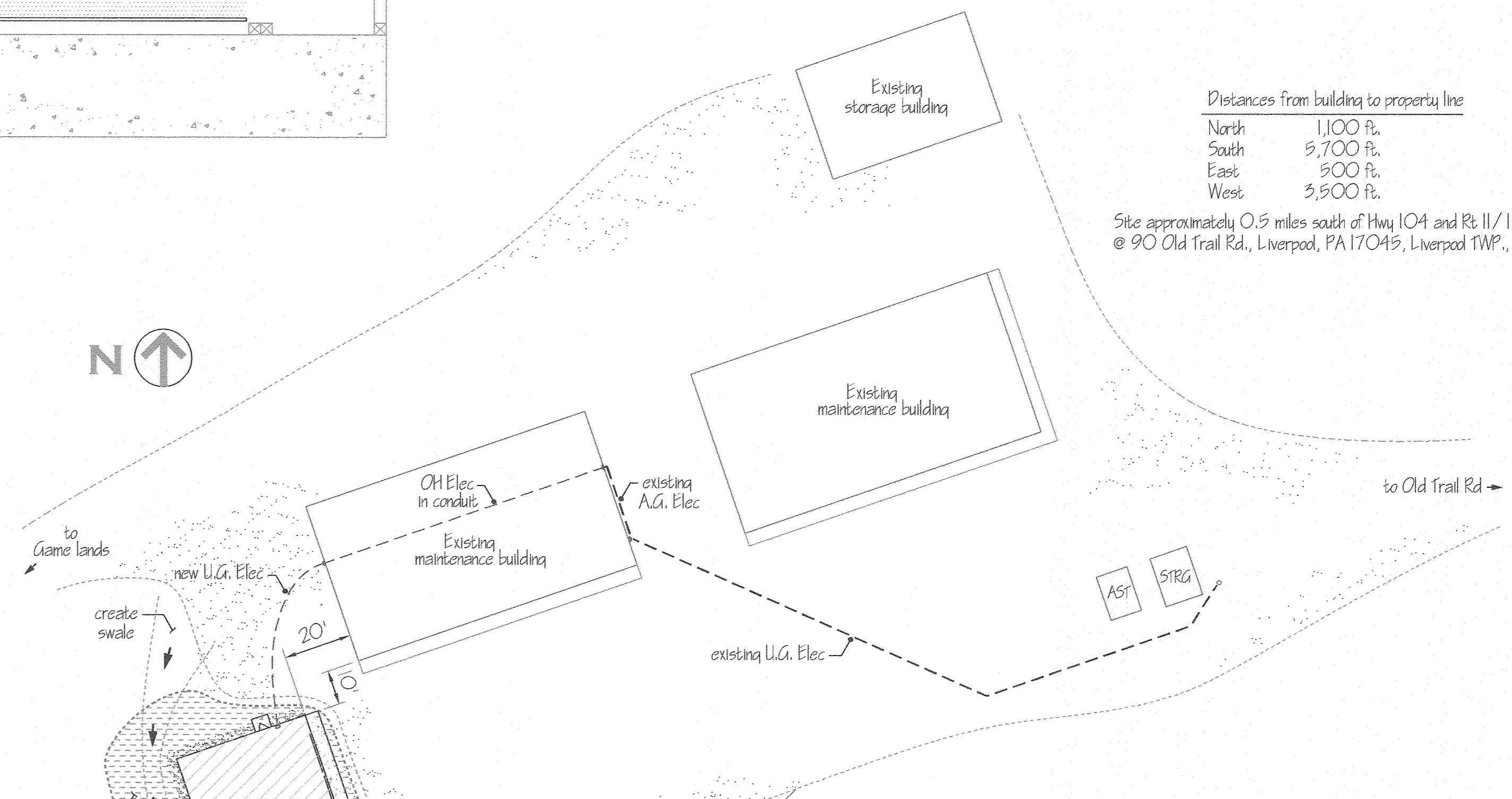
SITE PLAN 1" = 30'
